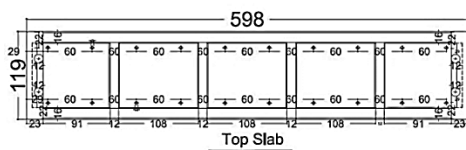
Top Slab
