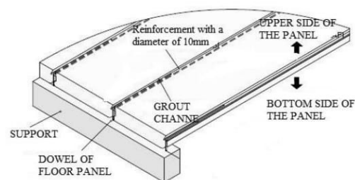
Figure 8. Floor panel connection.
